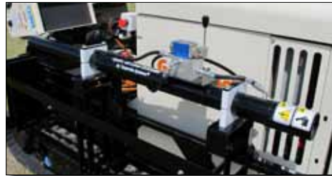
hydraulic liner extruder ...205501 (for 5 ft. rods) or 204258 (for 4 ft. rods)
