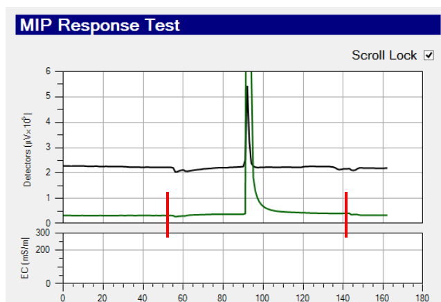
Figure 7: Response Test with a broad inject time
