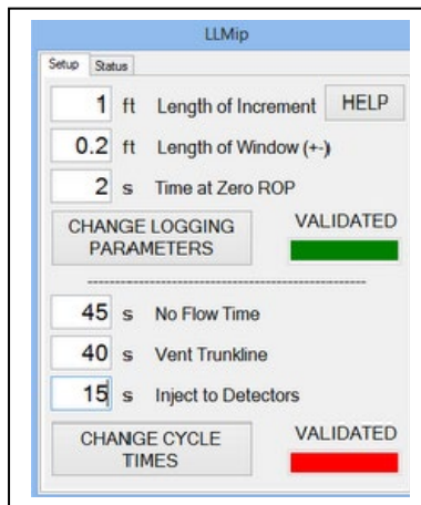
Figure 5: LL MIP Setup Screen
