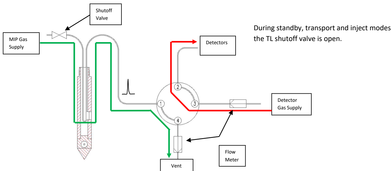
Figure 13: Transport of the sample to the surface with the valve still in the primary configuration.
